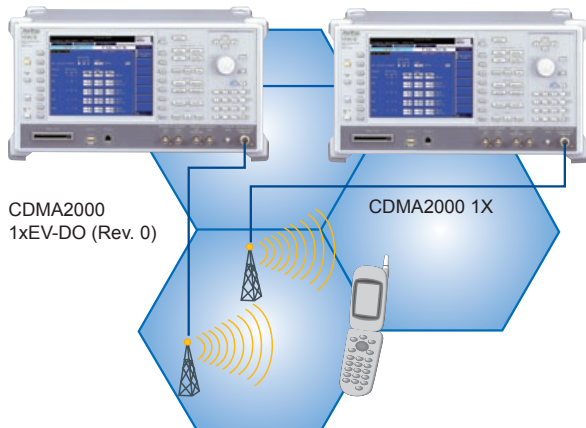
Sample MT8815B connection: When MT8815B is two sets
