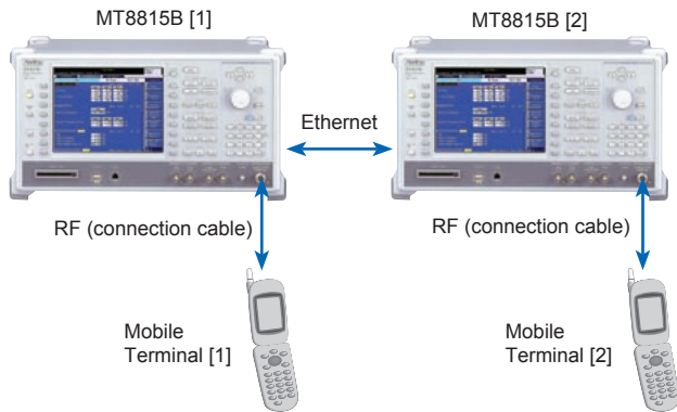
Sample MT8815B connection
